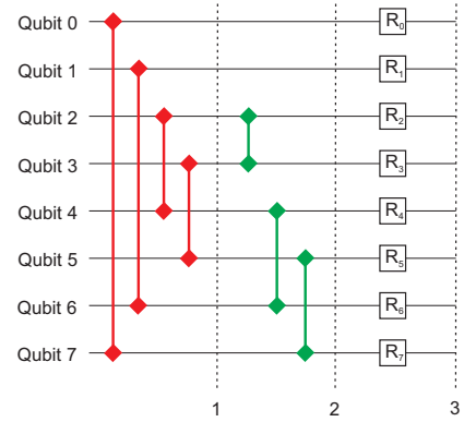
FIG. 5. Optimum circuit for preparing the graph state corresponding to Fig. 1.
